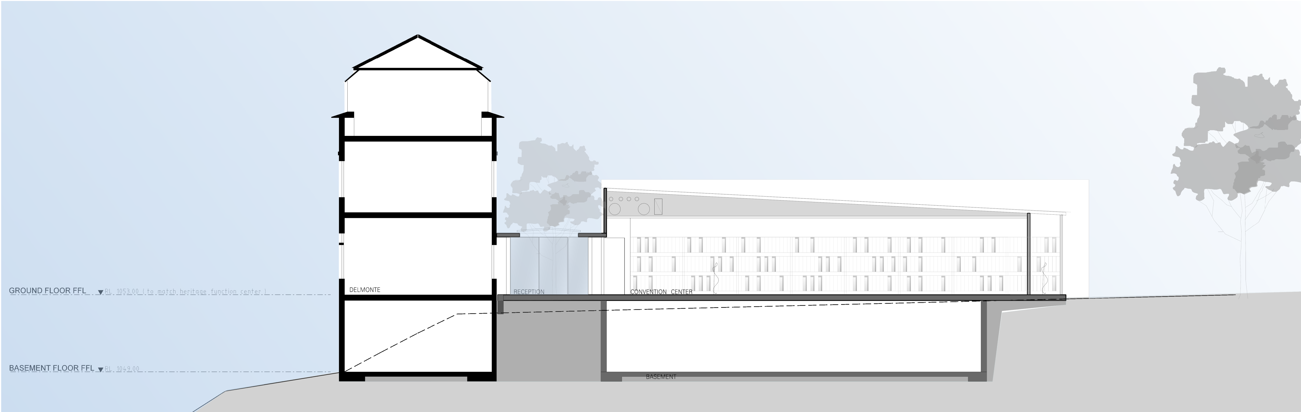
01 SECTION FF 1:100@A1
