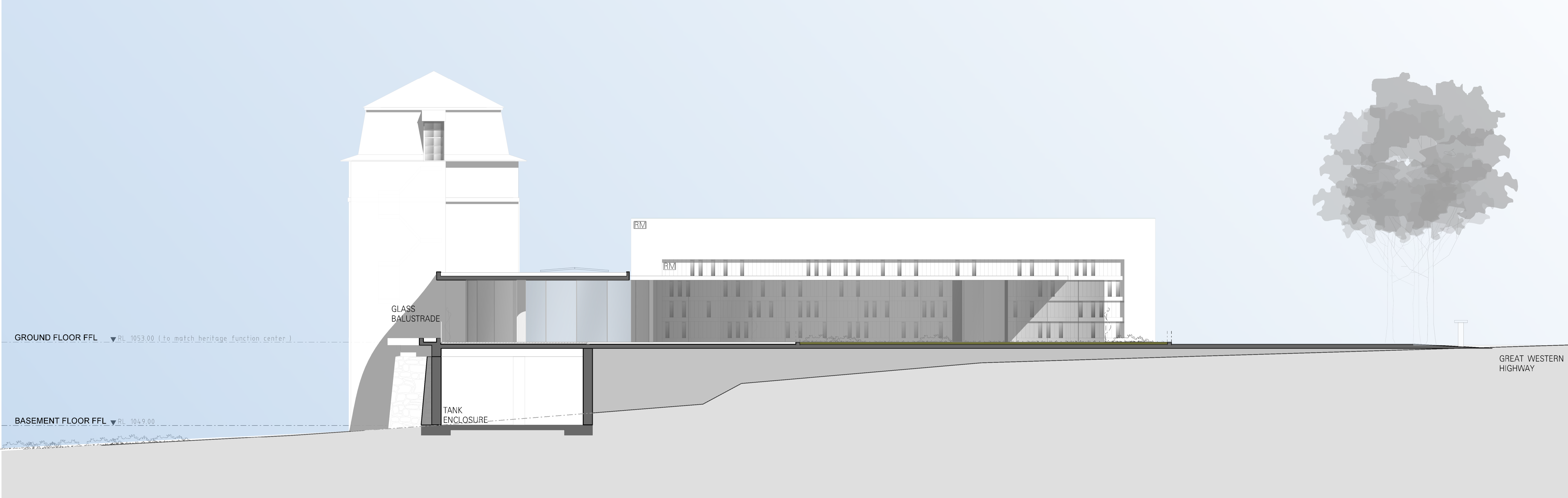
01 ELEVATION SOUTH 1:100@A1
